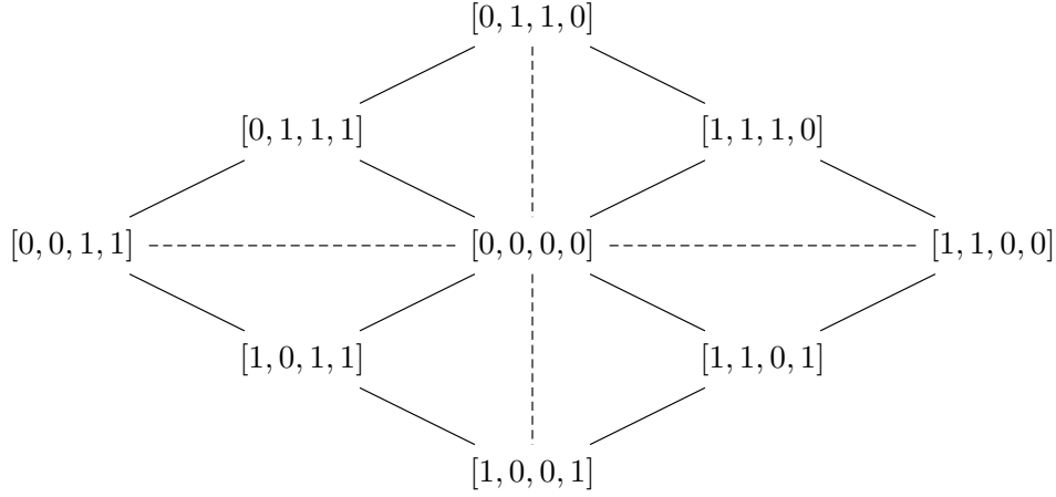
FIGURE 1. 1-ball around [0, 0, 0, 0] .
